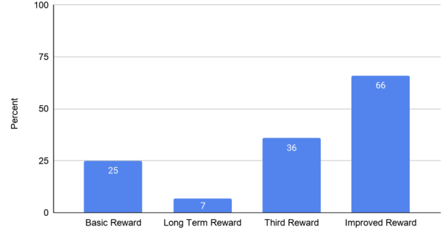
Fig. 2: Updated presentation chart comparing reward functions after one hour of training against three random bots. The improved reward was the strongest, reaching a 66% win rate.
